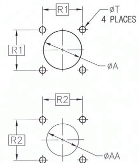
Mounting Cutouts
